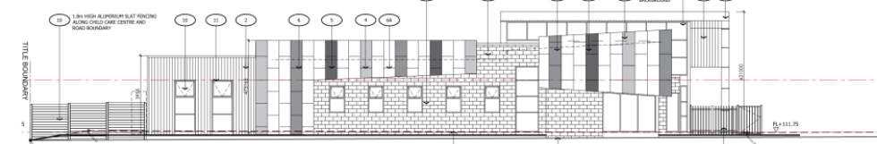
ELE 2 - EAST ELEVATION 1 (LEAKES ROAD) SCALE 1:100
