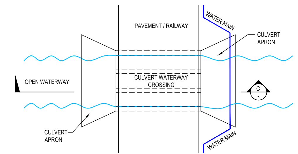
DETAIL B: PLAN VIEW, WATERWAY CROSSING
