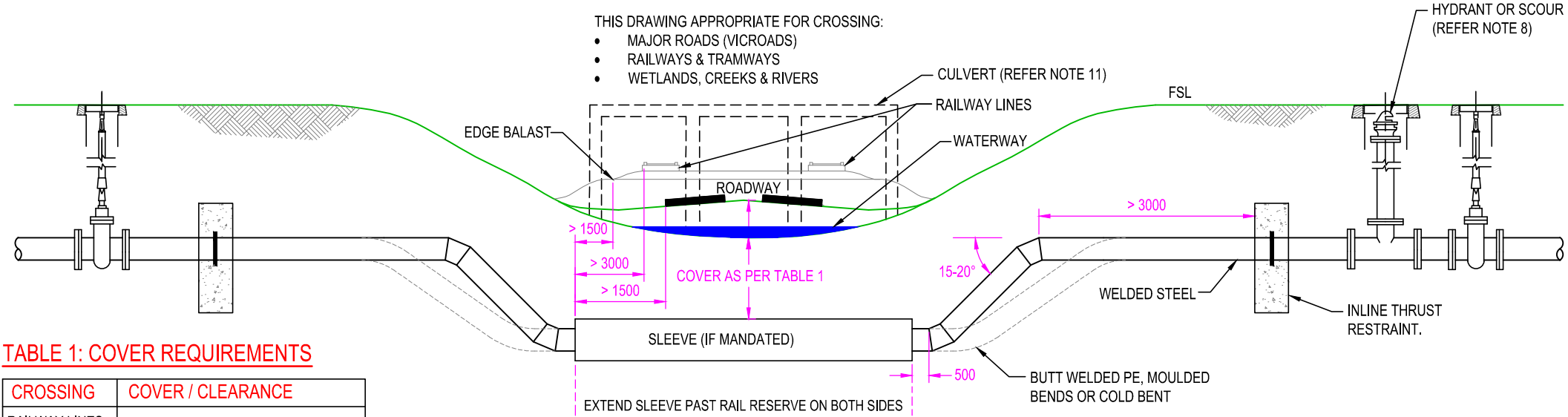
DETAIL A: SECTION VIEW, MAJOR ROAD / RAILWAY / TRAM / WATERWAY CROSSING
