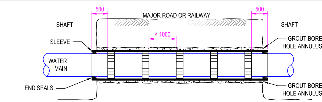
DETAIL E: TYPICAL SLEEVE INSTALLATION
